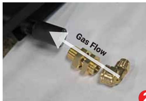
Installation of LP air mixer w/brass fitting
