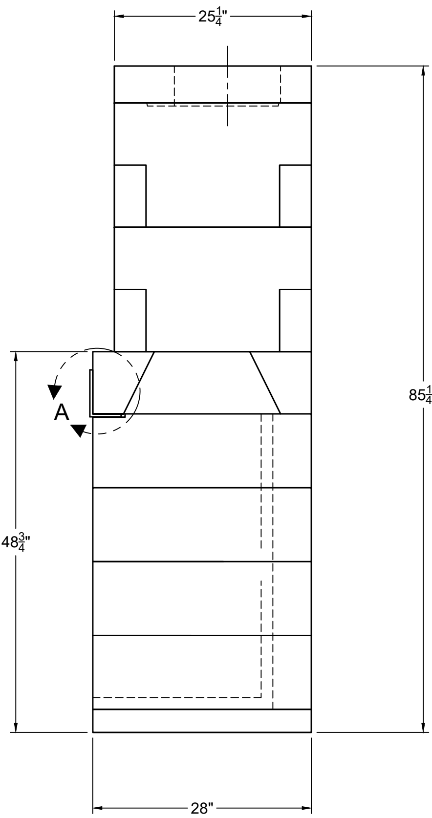
RIGHT-SIDE VIEW
