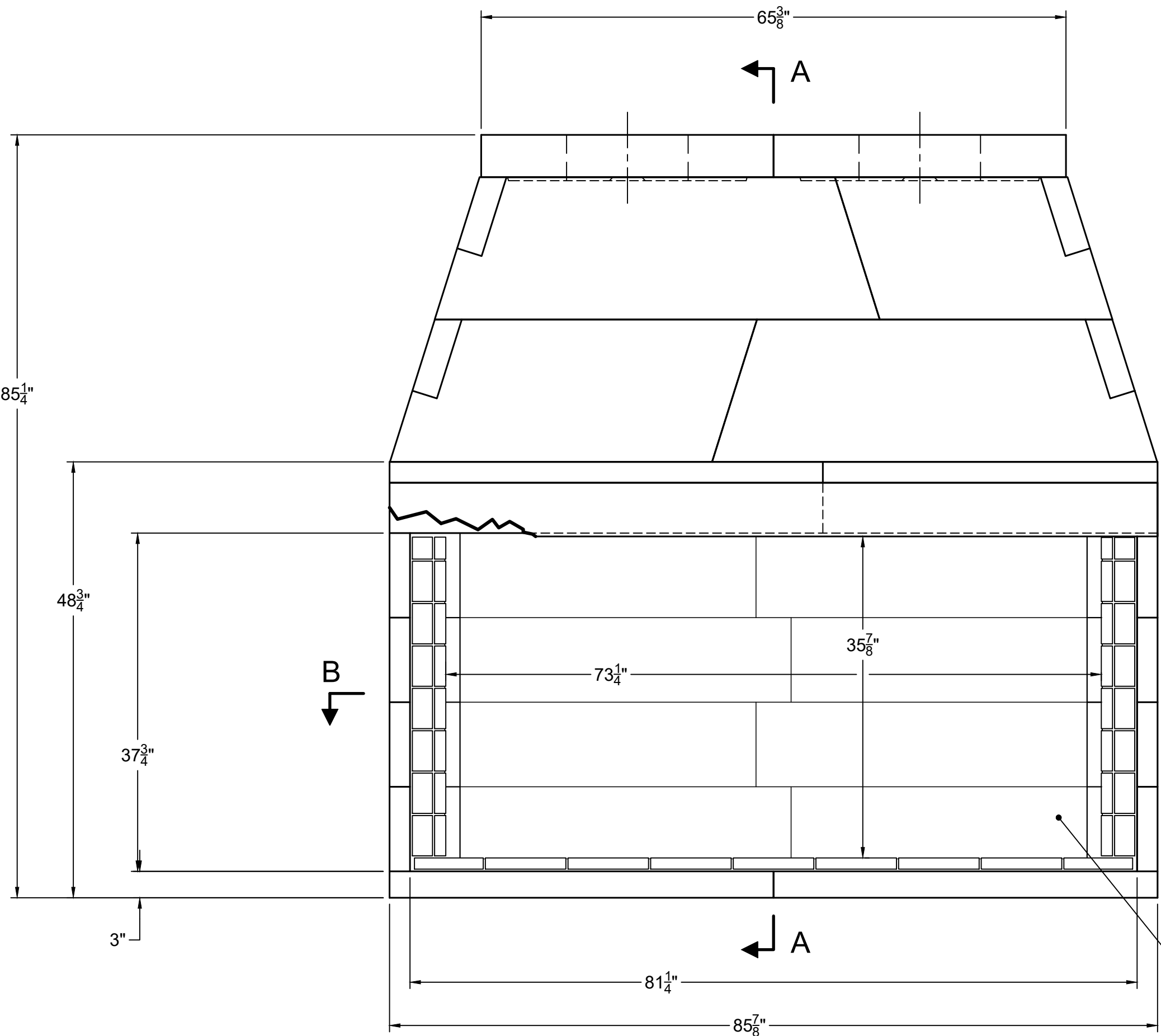
FRONT VIEW
