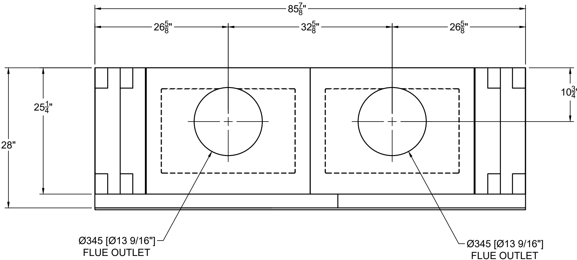
TOP VIEW
