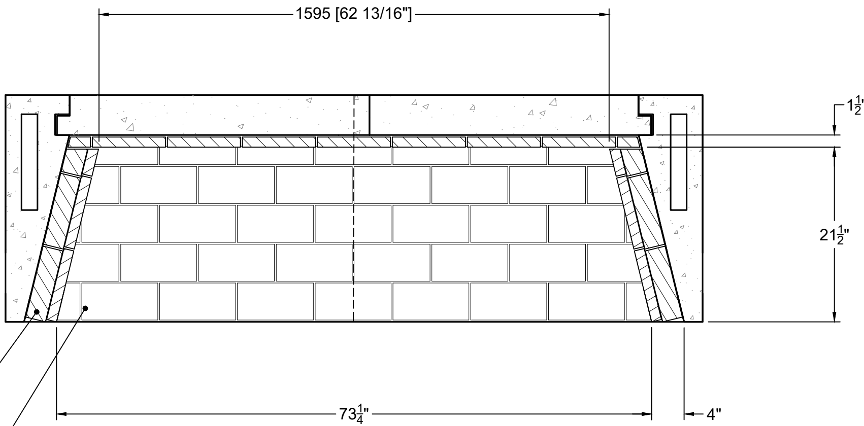
SECTION B-B HORIZONTAL FIREBRICK DETAIL
