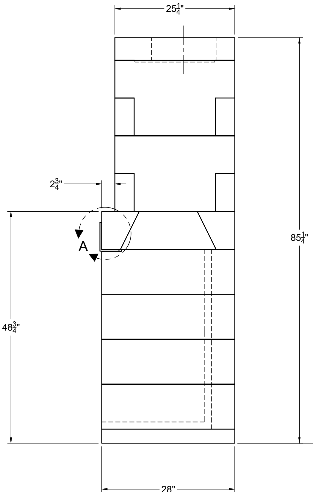
RIGHT-SIDE VIEW
