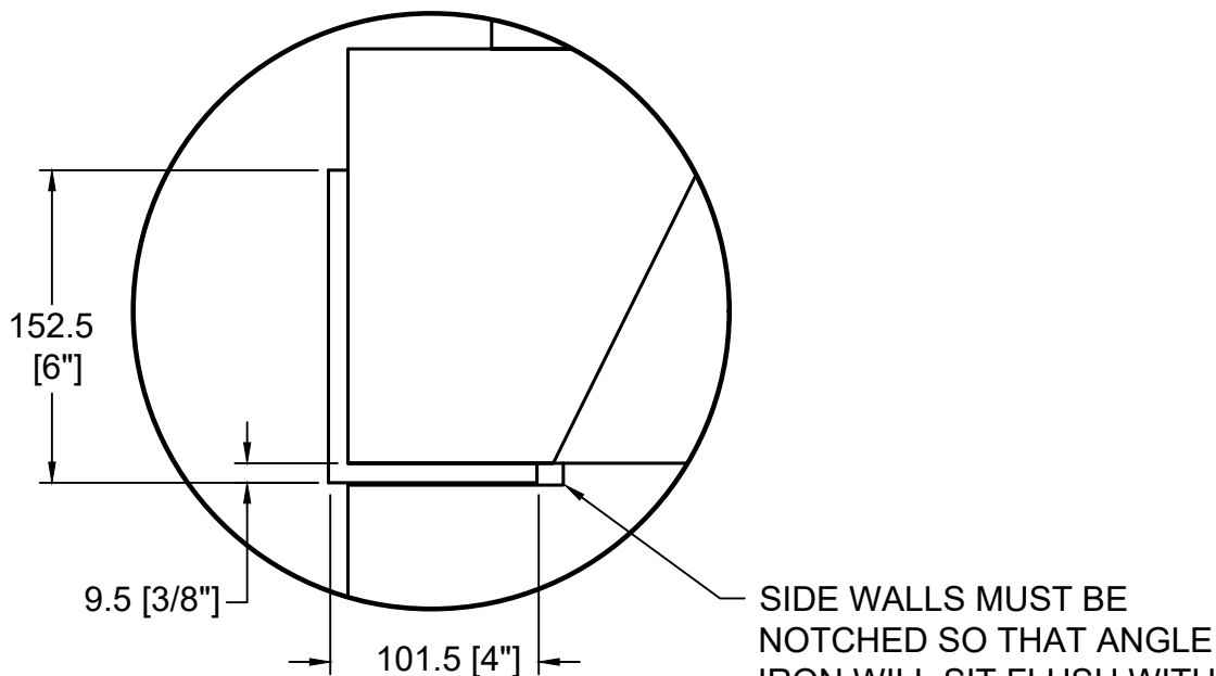
DETAIL A
