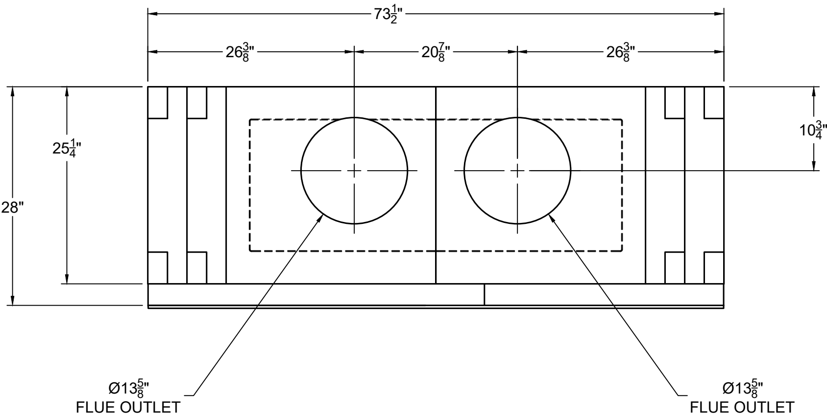
TOP VIEW
