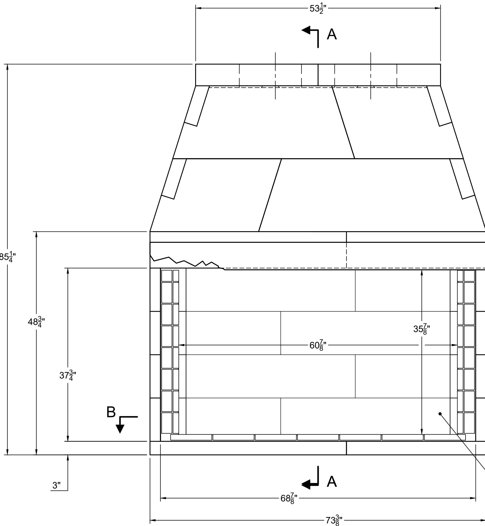
FRONT VIEW
