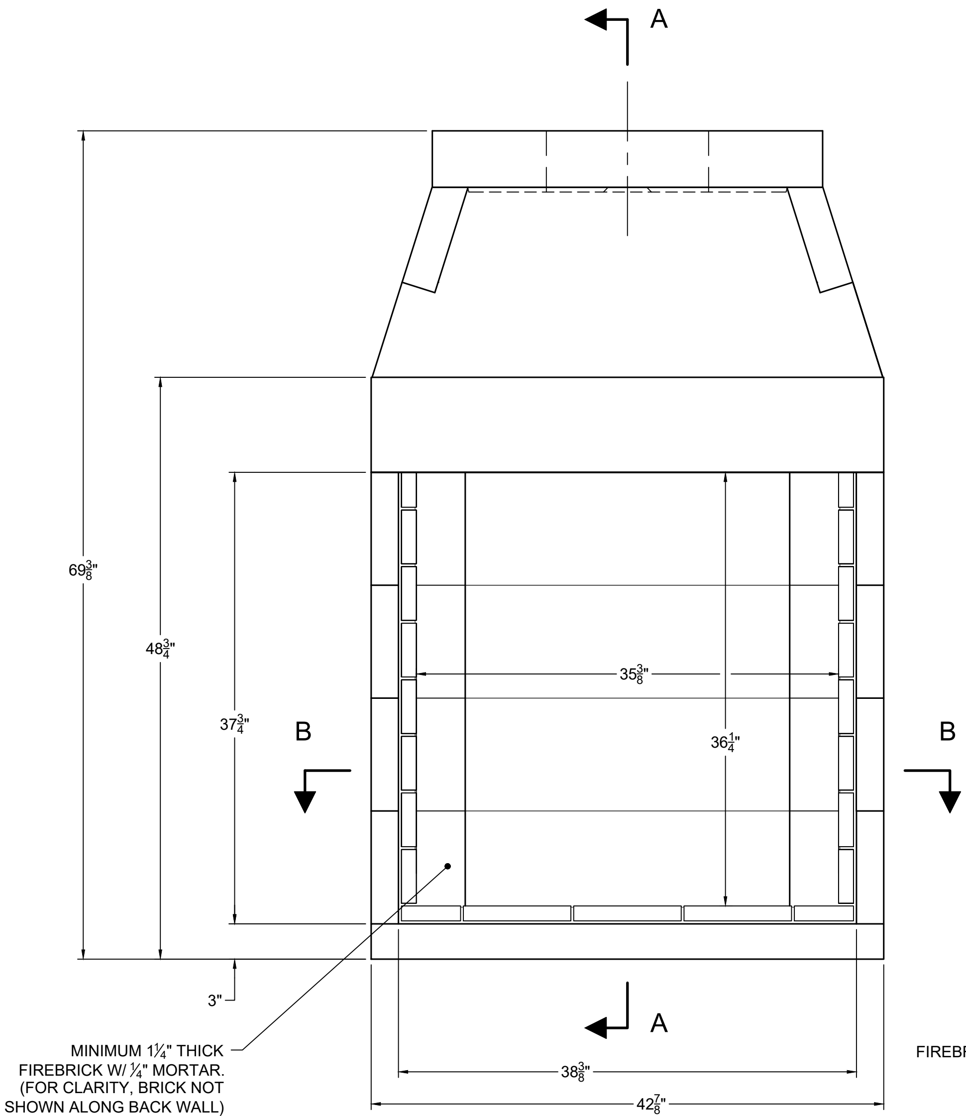
FRONT VIEW
