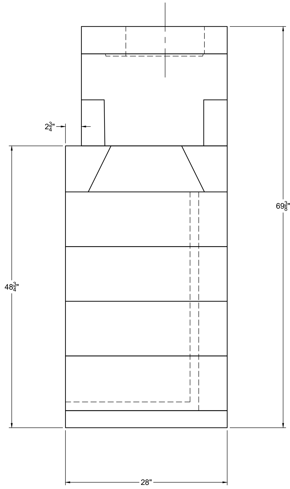
RIGHT-SIDE VIEW
