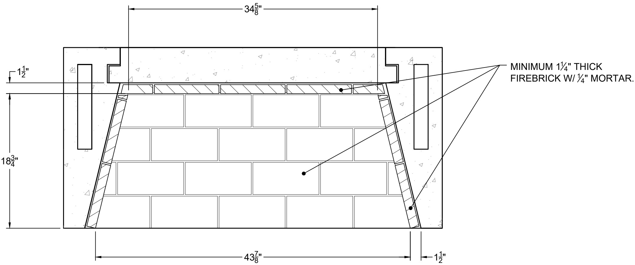
SECTION B-B HORIZONTAL FIREBRICK DETAIL
