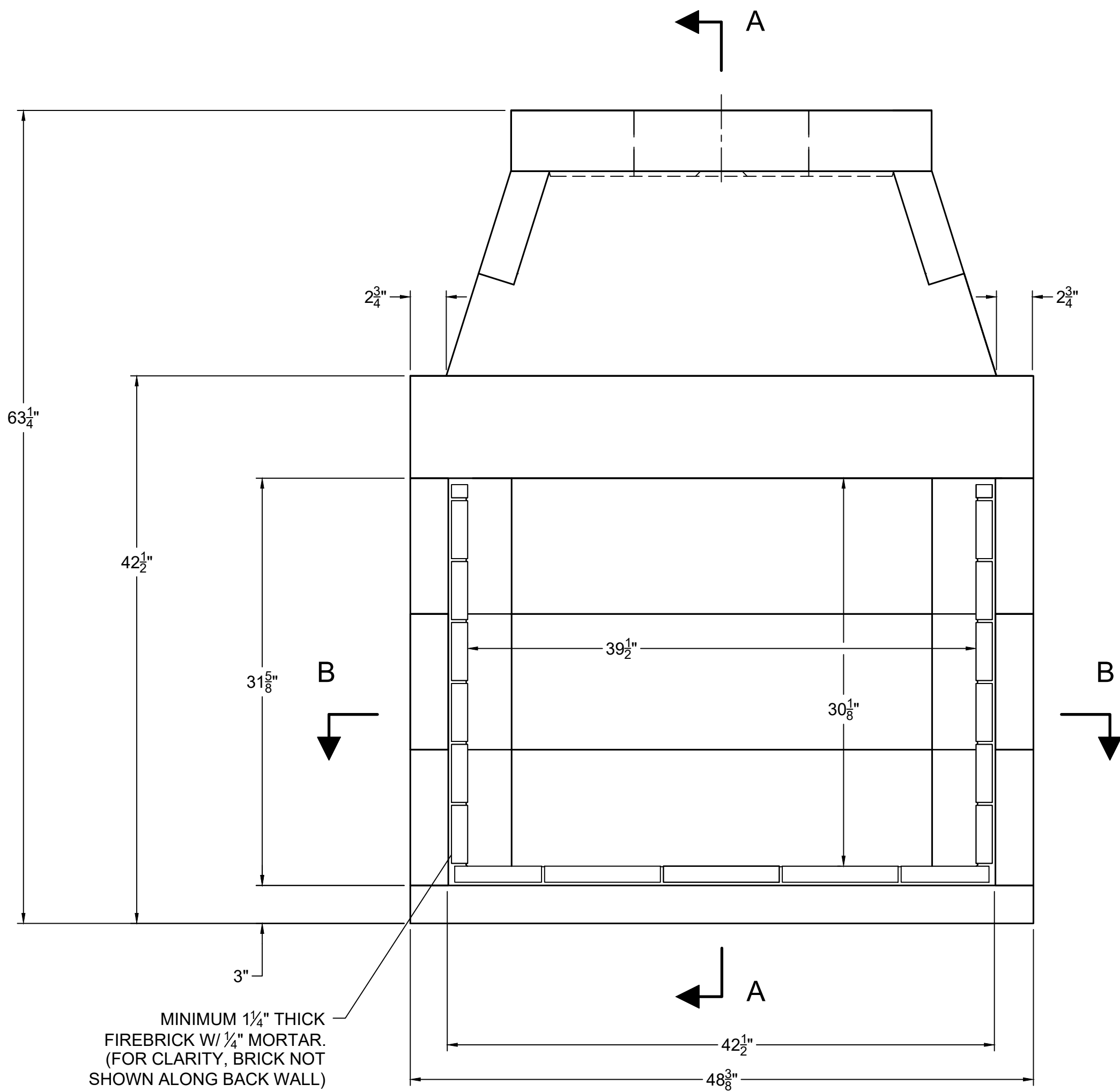
FRONT VIEW
