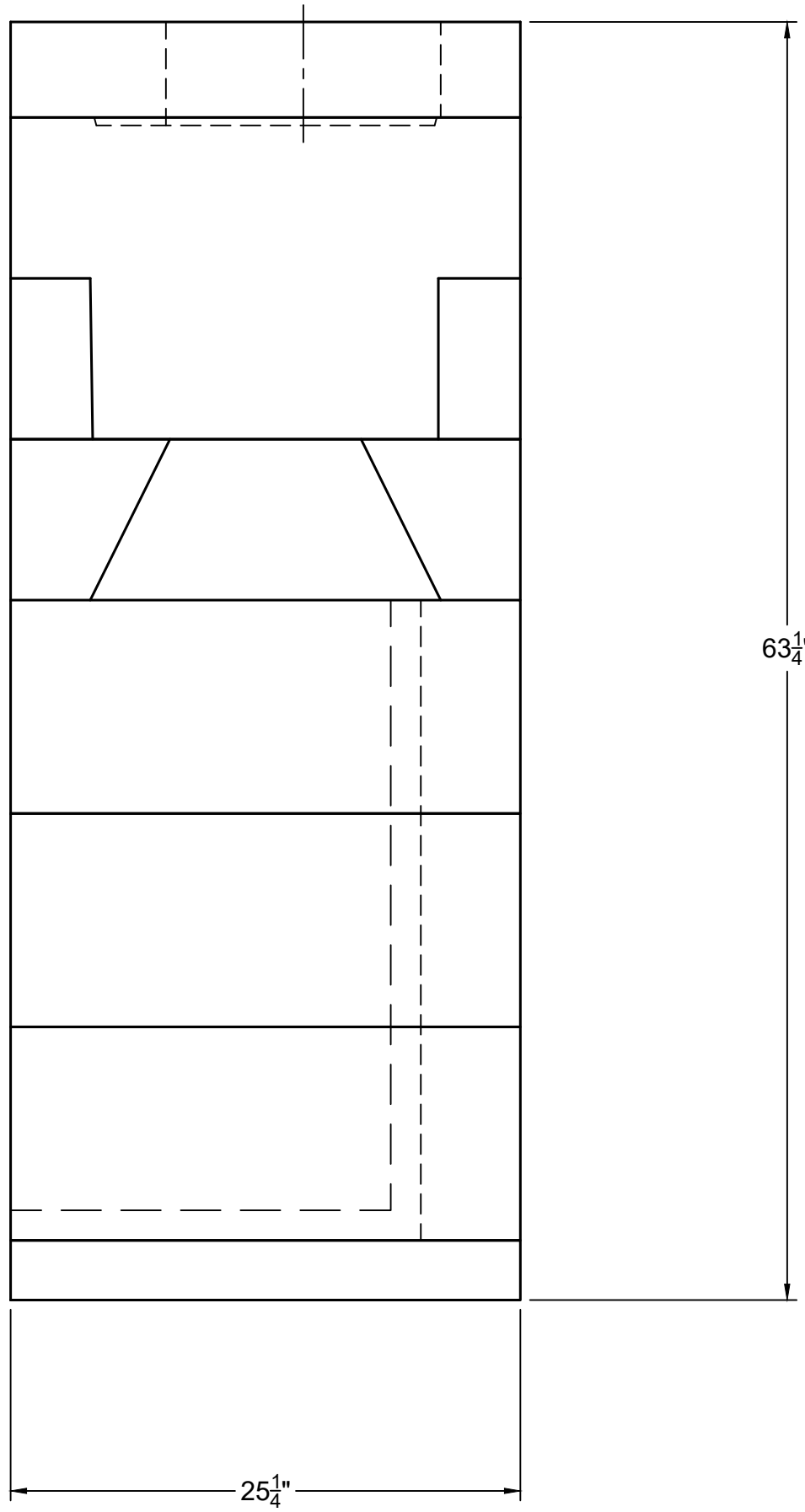
RIGHT-SIDE VIEW
