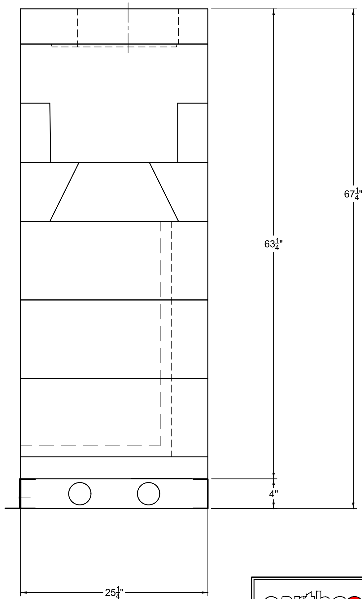
RIGHT-SIDE VIEW
