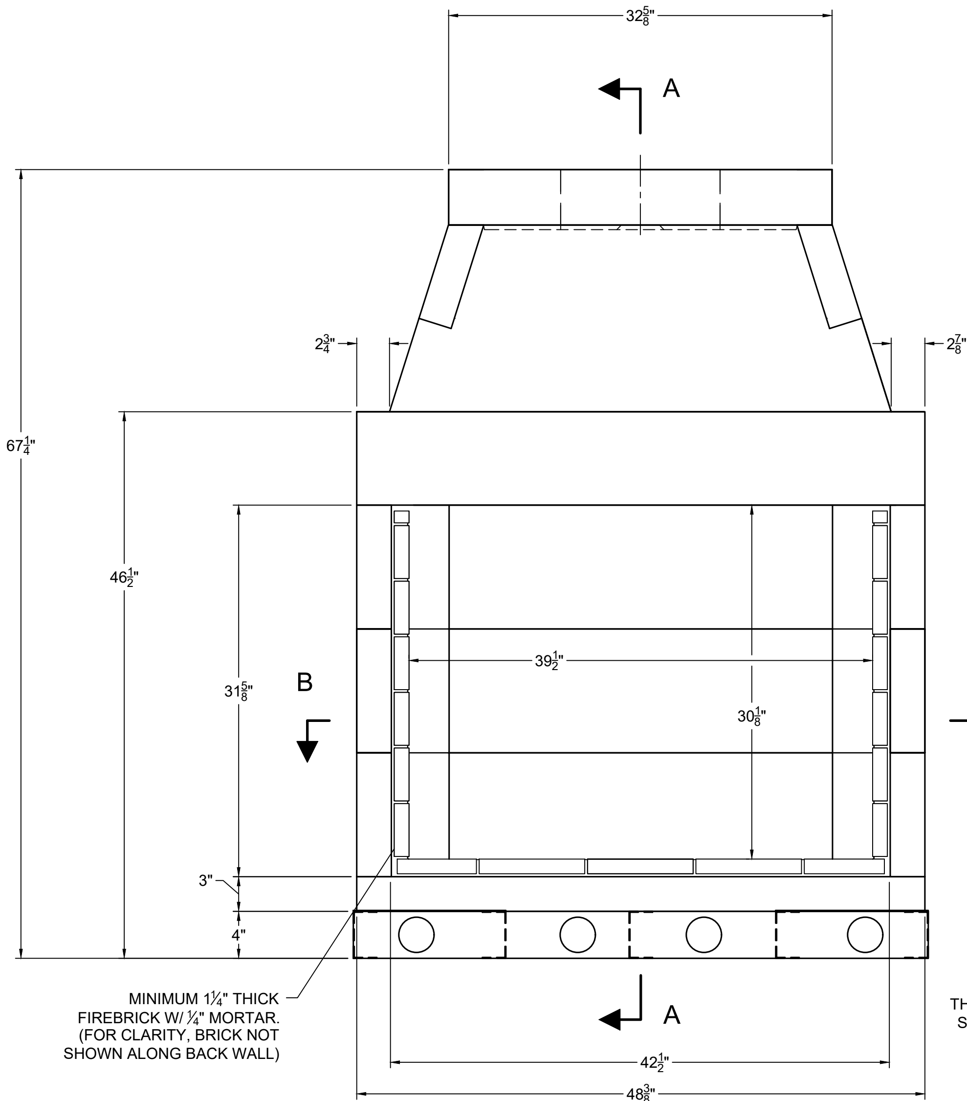
FRONT VIEW
